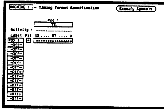
Figure 3-5. Pod Threshold
