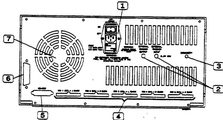
Figure 3-2. HP 1650B/51B Rear Panel
