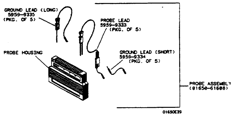
Figure 2-5. Probe Assembly
