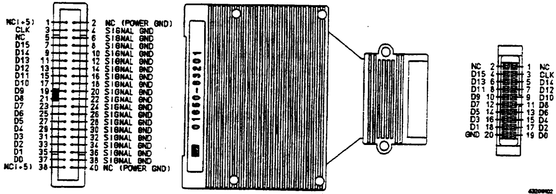
Figure 2-3. Termination Adapter Pinout
