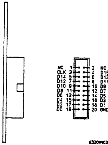
Figure 2-4. Connector Pinout (HP P/N 1251-8106)
